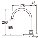
PA28JSX (Blister) Rp. 590.000,- • Ceramic cartridge type
