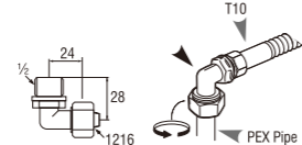
PT62-16 MALE ELBOW with NUT L16 X 1/2"
