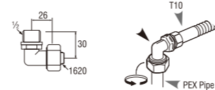
PT62-20 MALE ELBOW with NUT L20 X 1/2"
