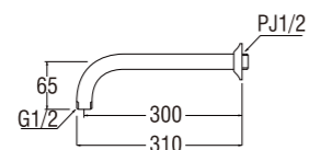
S104-63X2-MDP PIPE WALL SHOWER
