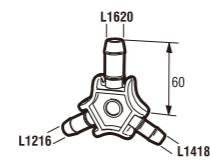
PT80 T-CALIBRATOR for PEX PIPE
