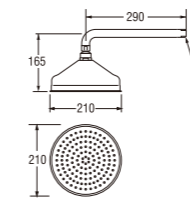
PS25-L RELAXATION WALL SHOWER
