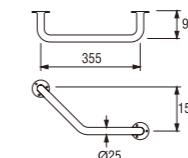
WN59 GRIP BAR
