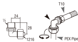
PT62-16 MALE ELBOW with NUT L16 X 1/2"
